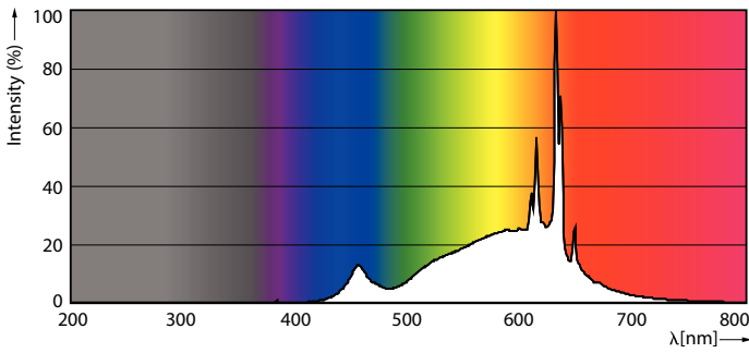
Spectral Power Distribution Colour - 5R20/PER/927/P/E26/DIM 6/1FB T20
