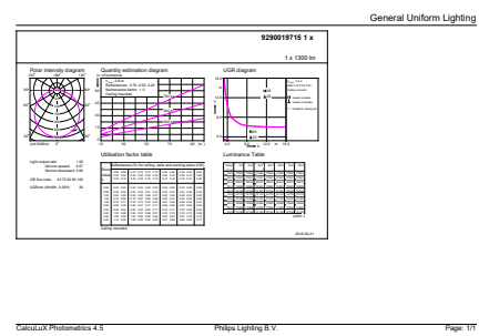
General uniform lighting - UFO LEDBulb 15W E27 6500K 230V 1CT/6
