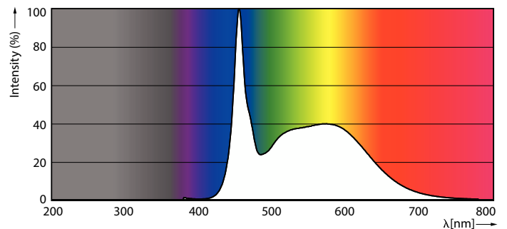
Spectral Power Distribution Colour - Master LEDTube 1200mm 12.5W 865 T8 W JP
