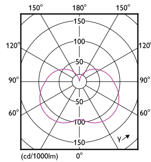
Light Distribution Diagram - LED PLC 7.5W 830 2P G24d
