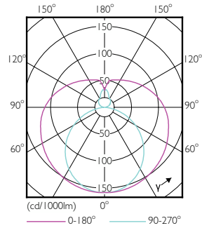
Light Distribution Diagram - CorePro LEDtube UN 1200mm HO 18W830 T8
