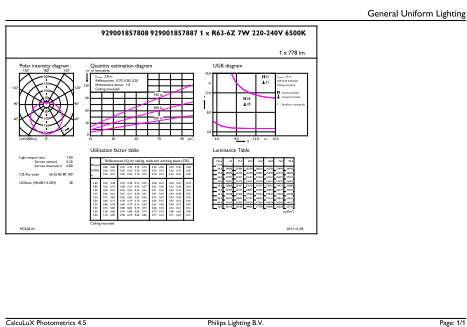
Accent Lighting Spots - LED 7W E27 6500K 230V R63 AU
