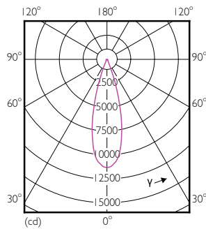
Light Distribution Diagram - Master LED PAR30L 32W 30D 840 220V
