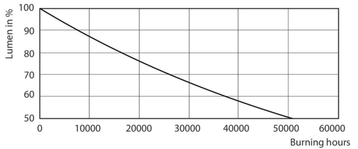
Lumen Maintenance Diagram - MAS LED spot VLE D 5-65W GU10 940 36D
