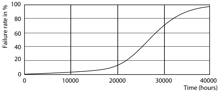
25K LED Lumen Maintenance Diagram - MAS LED spot VLE D 3.7-35W GU10 940 60D
