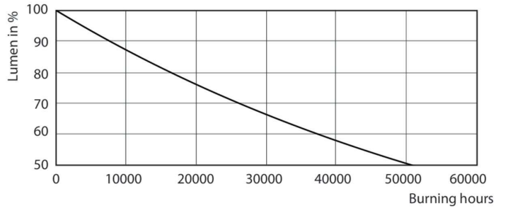
25K LED Lumen Maintenance Diagram - MAS LED spot VLE D 3.7-35W GU10 940 60D
