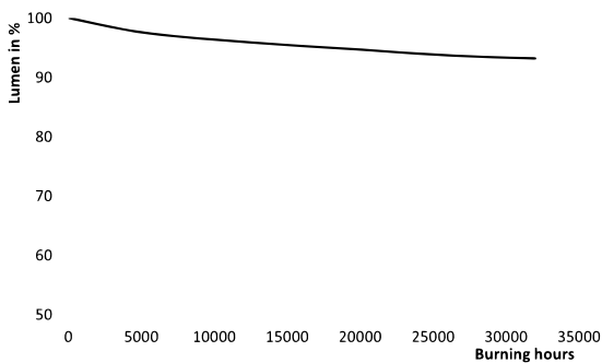
Lumen Maintenance Diagram - MASTER SON-T PIA PLUS 150W E E40 1SL/12
