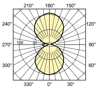
Light Distribution Diagram - MASTER SON-T PIA PLUS 150W E E40 1SL/12
