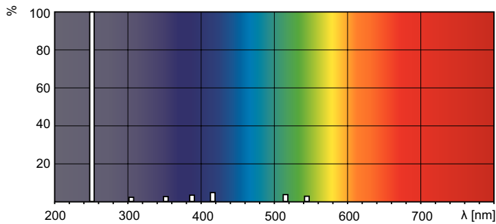
Spectral Power Distribution Colour - TUV 320W XPT SE UNP/20
