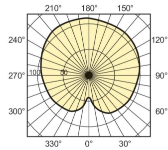
Light Distribution Diagram - HPI-T Plus 250W/645 E40 1SL/12
