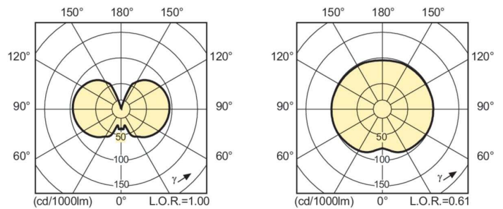
Light Distribution Diagram - MASTERC CDM-TC Elite 70W/942 G8.5 ICT
