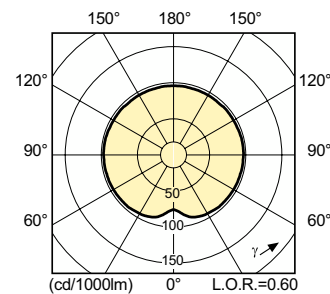
Light Distribution Diagram - MASTERC CDM-T Elite 70W/942 G12 1CT
