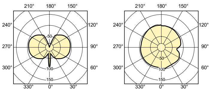
Light Distribution Diagram - MASTERC CDM-TC Elite 35W/930 G8.5 ICT/12
