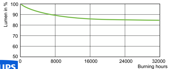
Maintenance Diagram - MASTER GreenPower 600W 480V E40 1SL/12
