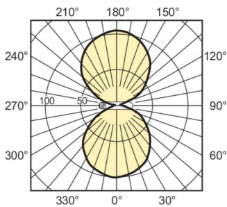
Light Distribution Diagram - MASTER GreenPower 600W 480V E40 1SL/12
