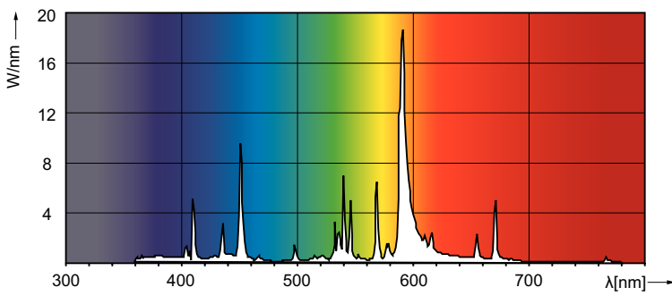
Spectral Power Distribution Colour - MASTER MHN-FC 2200W/640 400V XW
