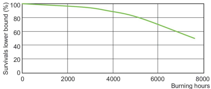
LDLE_MHN-FC_2200W_640-Life expectancy diagram
