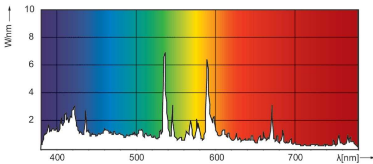
Spectral Power Distribution Colour - MASTER MHN-LA 1000W/956 230V XWH
