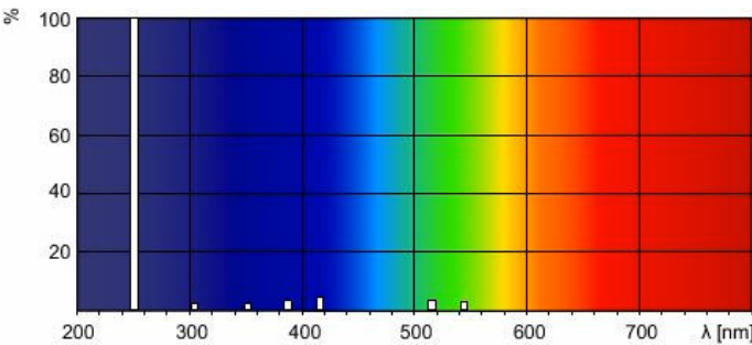
Spectral Power Distribution Colour - TUV 25W 1SL/25
