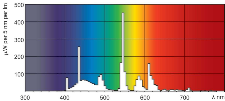
Spectral Power Distribution Colour - MASTER PL-L 24W/865/4P 1CT/25_APR
