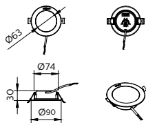
cut-out: Ø75 - Ø85 mm
