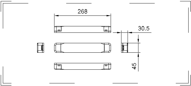
ST307Z 150W PSU driver
