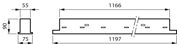
Recessed VPC_W&L120_sensor/IP
