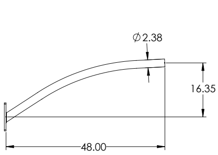
4ft Arm
