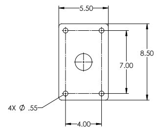
Mount plate
