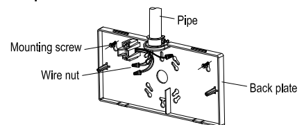
Wall mount-Top Power Feed
