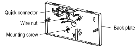
Wall mount-Top Power Feed
