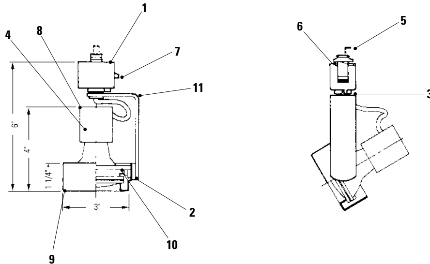
Fixture MOL=6 3/4"
